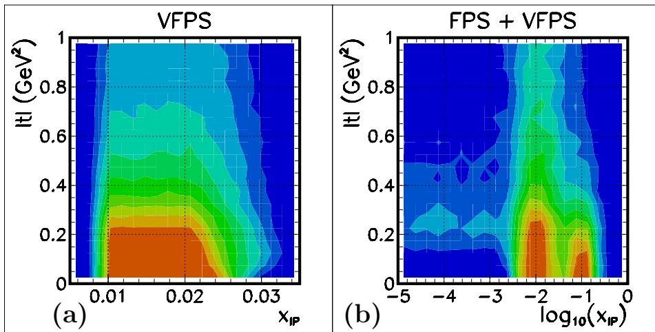
Fig. 1. Illustration of the acceptance regions of (a) the H1 VFPS and (b) the H1 VFPS and FPS combined. Acceptances of above 90% are coded red, with each subsequent colour coding covering a range of 10%.
