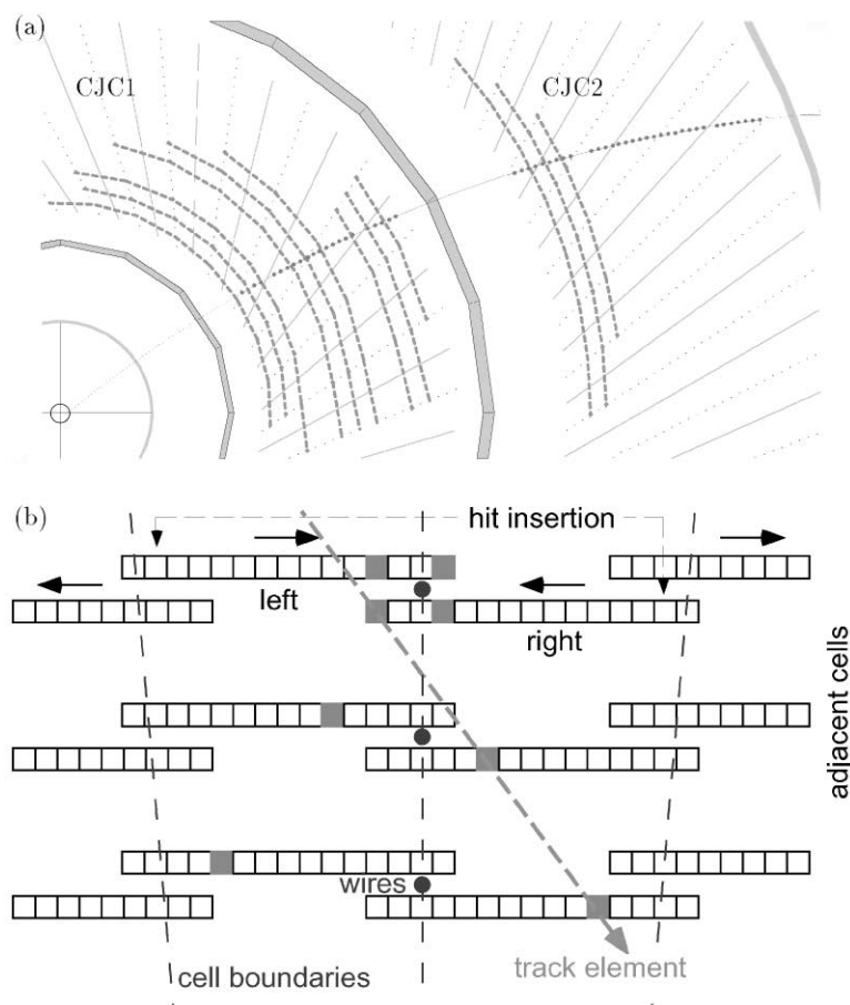
Fig. 1. (a) r\phi view of the central drift chamber showing a track passing through. The position of the sense wires, the cathode planes and the chamber boundaries are also shown. The four groups of wire planes used by the FTT are indicated by the thick dashed lines. (b) Schematics showing the hit pattern recognition of track segments using shift registers at the first trigger level L1.
