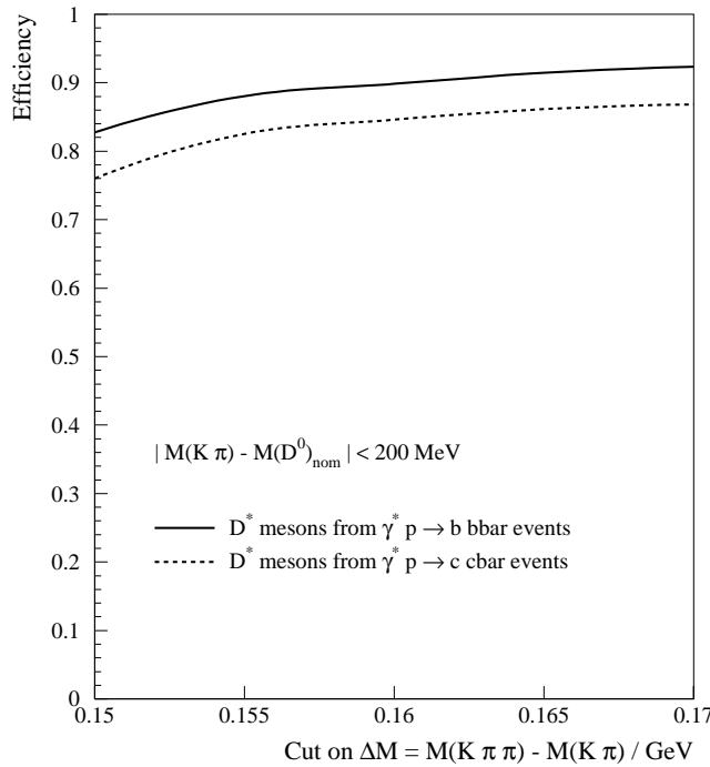
Figure 1: Estimated efficiencies for D^* mesons in DIS using the proposed trigger for |M(K\pi) - M(D^0)| < 200 MeV and various choices of cut on \Delta M . The efficiencies are relative to a sample of simulated events in which the selection criteria on the polar angles and transverse momenta of the D^* and its decay products of [2] are applied. A comparison is made between D^* mesons produced directly in the process \gamma^* p \rightarrow c \bar{c} and those produced as part of the decay chain following the hard process \gamma^* p \rightarrow b \bar{b} .
