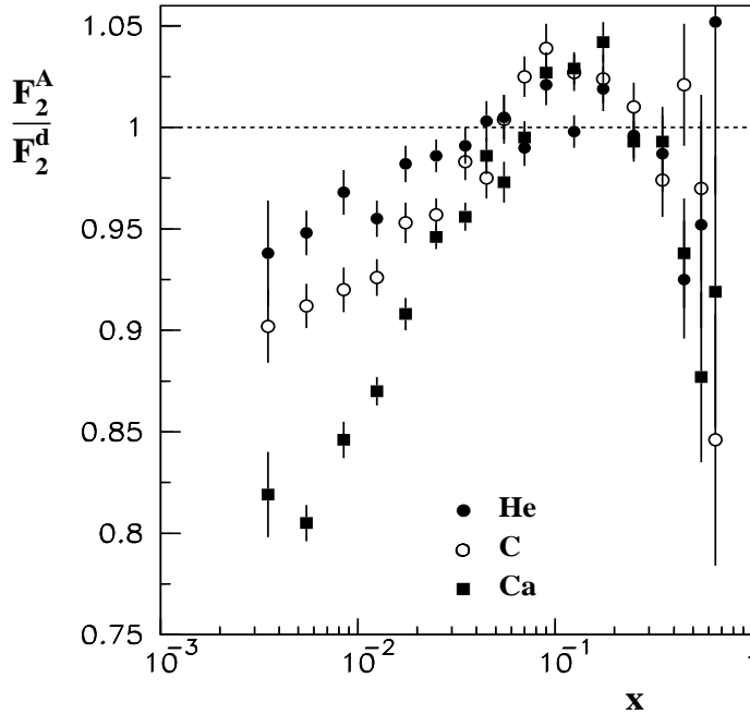
Figure 1.4.1: NMC data [131] for the structure function ratio F_2^A/F_2^d per nucleon for ^4\text{He} , ^{12}\text{C} and ^{40}\text{Ca} for Q^2 \geq 0.7 \text{ GeV}^2 . THERA would extend these measurements by three orders of magnitude to x \simeq 10^{-5} .
