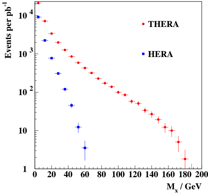
Figure 1.2.7: Event yields per unit luminosity for the process ep \rightarrow eXp after applying the quoted selection criteria at THERA (920 GeV protons, 250 GeV electrons) and HERA. The yields are shown as a function of the mass M_X and are based on an ad hoc extrapolation of a QCD fit to HERA data [42].
