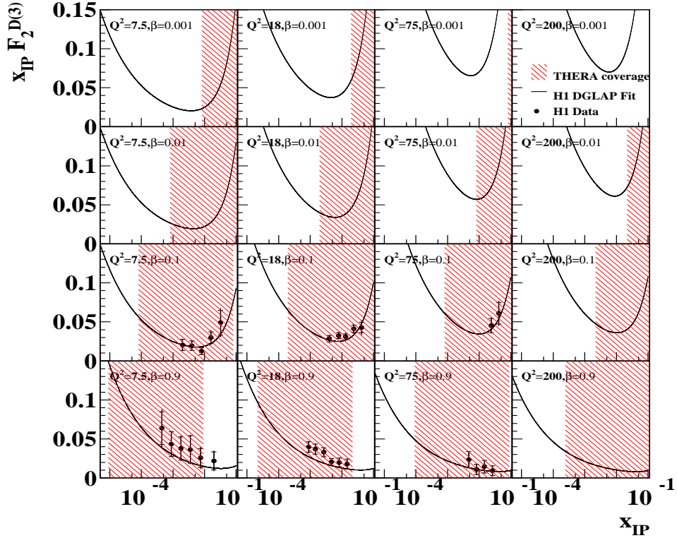
Figure 1.2.6: Illustration of the kinematic coverage for measurements of F_2^{D(3)}(x_{IP}, \beta, Q^2) at HERA and at THERA. The accessible x_{IP} range is shown for selected values of \beta and Q^2 . Appropriate HERA data points from [42] are also shown. The curves are extrapolations of QCD fits to data with \beta < 0.65 from [42]. The shaded areas show the region of extended coverage at THERA (920 GeV protons, 250 GeV electrons).
