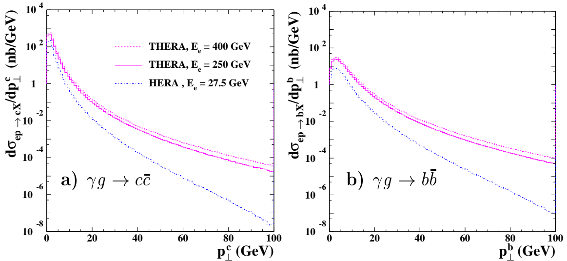
Figure 1.2.11: The contribution of photon–gluon fusion to the differential cross sections d\sigma/dp_\perp for (a) charm and (b) beauty production calculated in NLO QCD for Q^2 < 1\text{ GeV}^2 . The solid and dashed violet curves show the predictions for THERA operation with an electron energy of 250\text{ GeV} and 400\text{ GeV} , respectively, and E_p = 920\text{ GeV} . The predictions for the HERA case are indicated by the dash-dotted blue curves.
